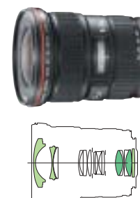
EF 16-35mm f/2.8L USM
